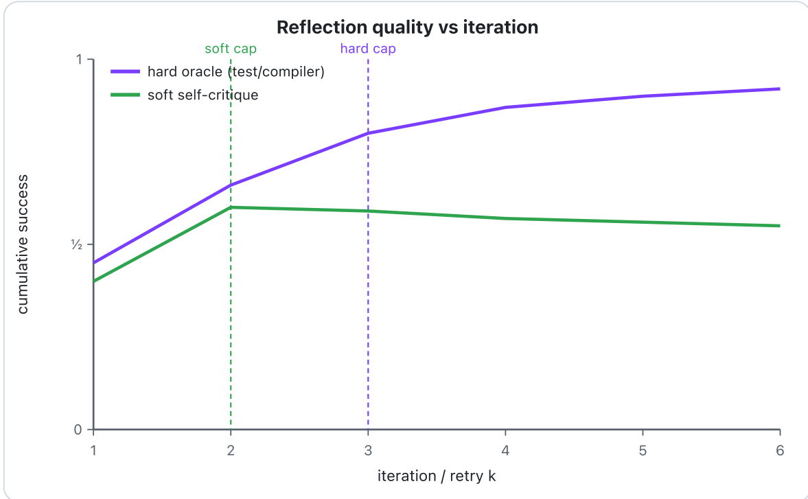
Figure 5. A hard oracle (test, compiler) keeps improving and saturates late; soft self-critique plateaus and dips after two passes (R8). The \sim 2 soft / \sim 3 hard caps are fabius's operational heuristics.
