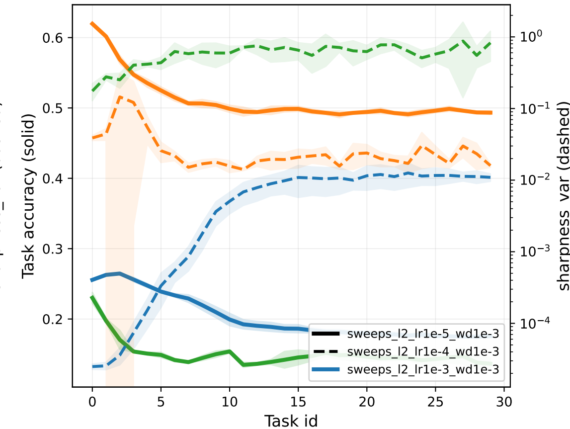
L2 (first 30 tasks)
