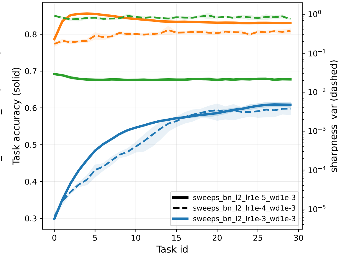
BN+L2 (first 30 tasks)
