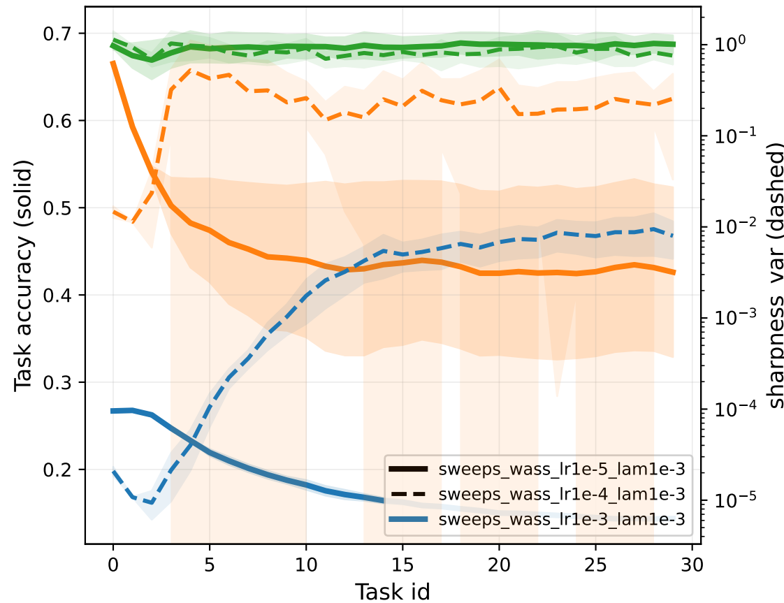
Wasserstein (first 30 tasks)
