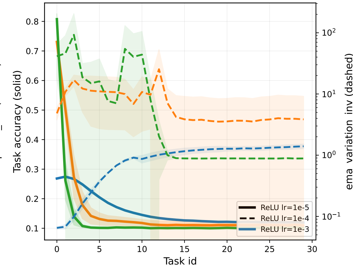
ReLU (first 30 tasks)
