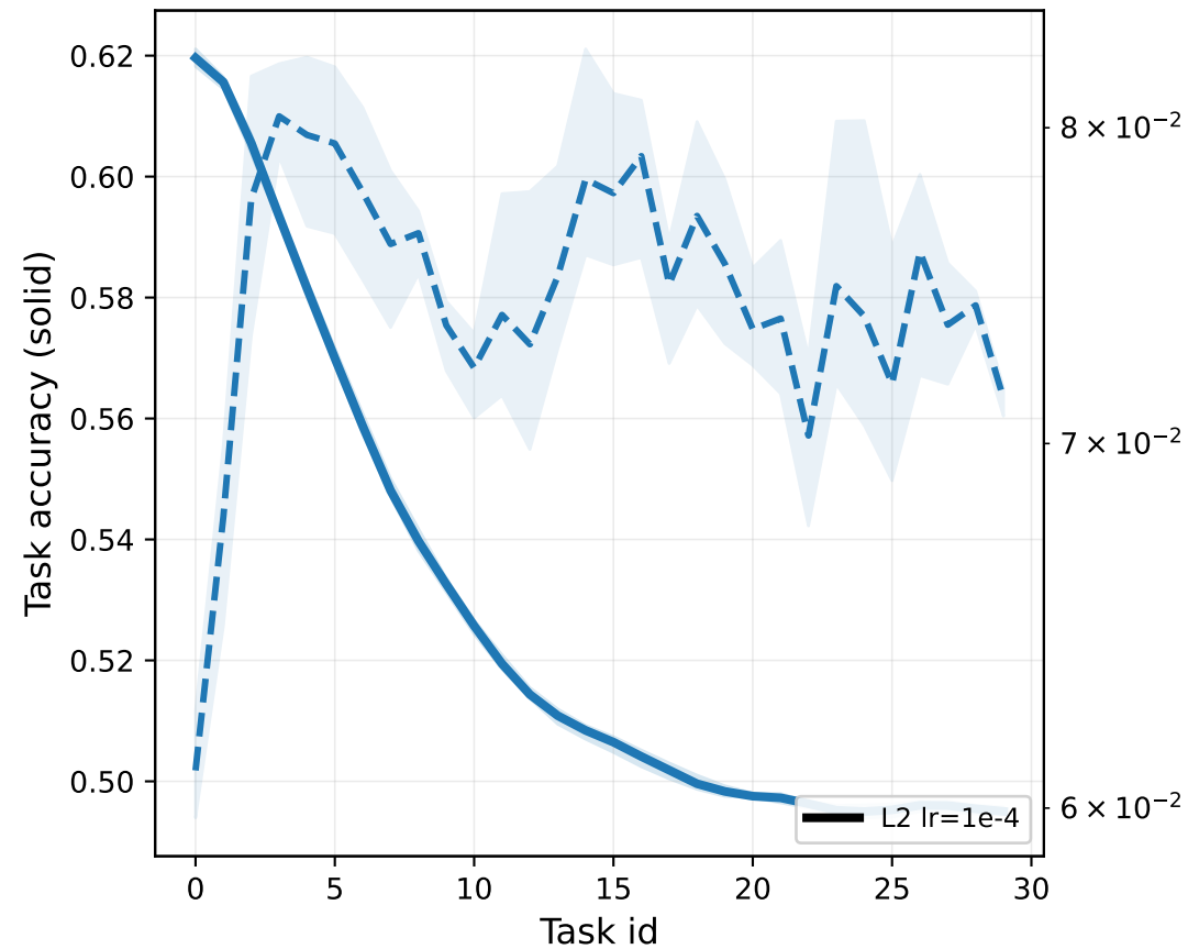
L2 (first 30 tasks)
