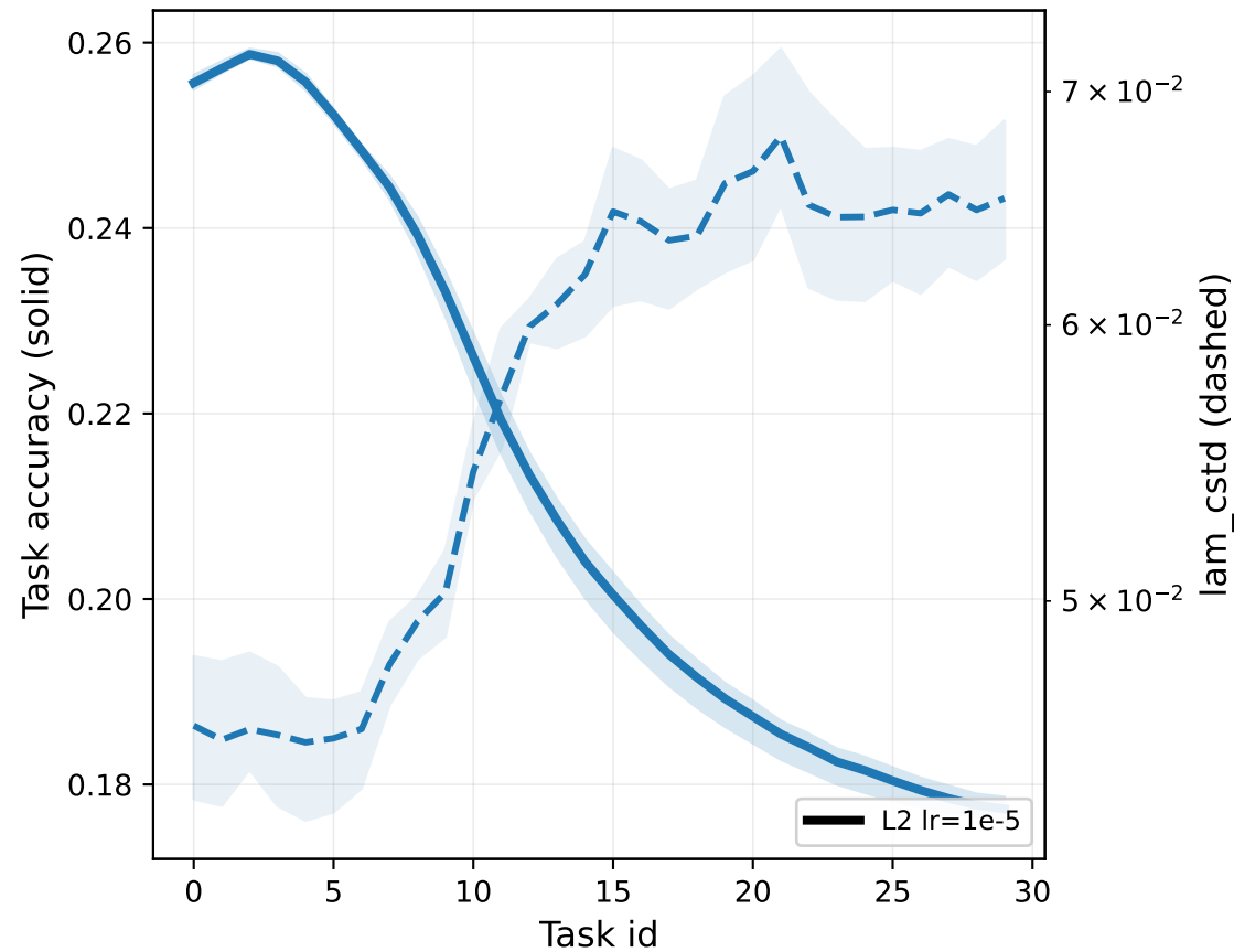
L2 (first 30 tasks)
