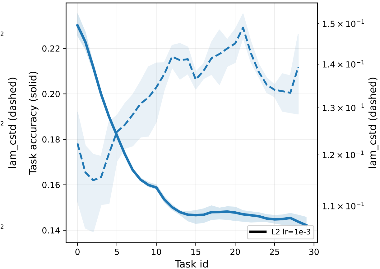
L2 (first 30 tasks)
