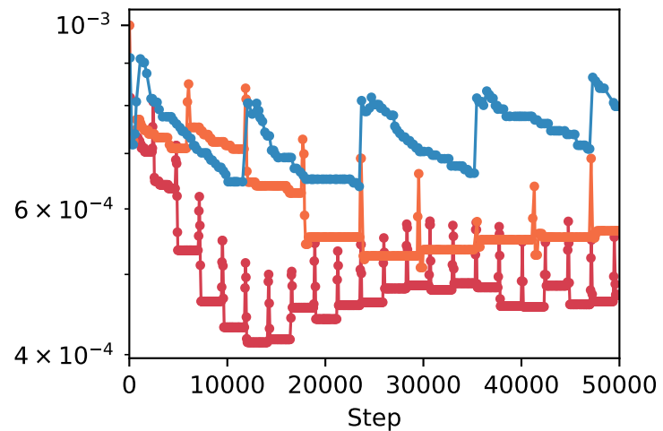
Wasserstein ( \lambda = 0.001 )
