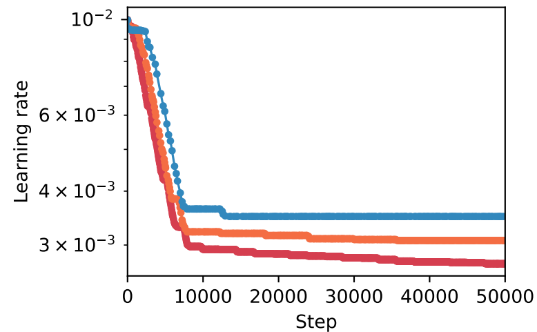
CReLU (lr=0.01)
