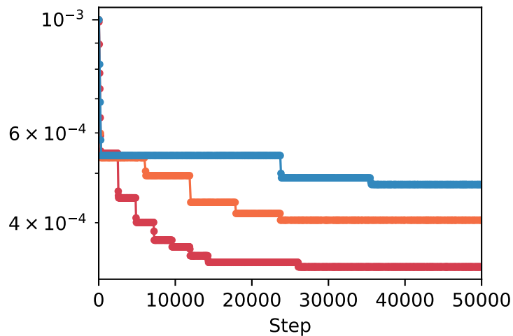
L2 ( \lambda = 0.001 )
