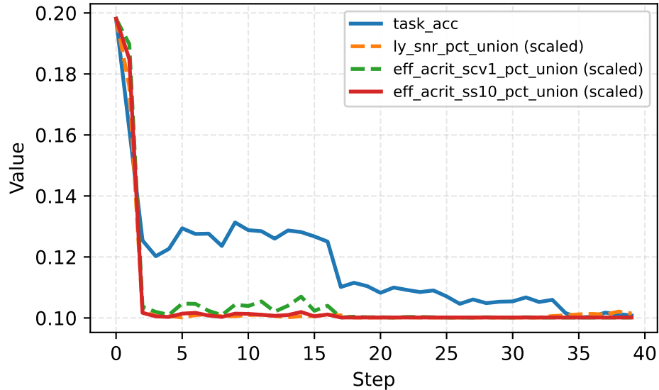
Run C ka / l2_f_1e-3_250
