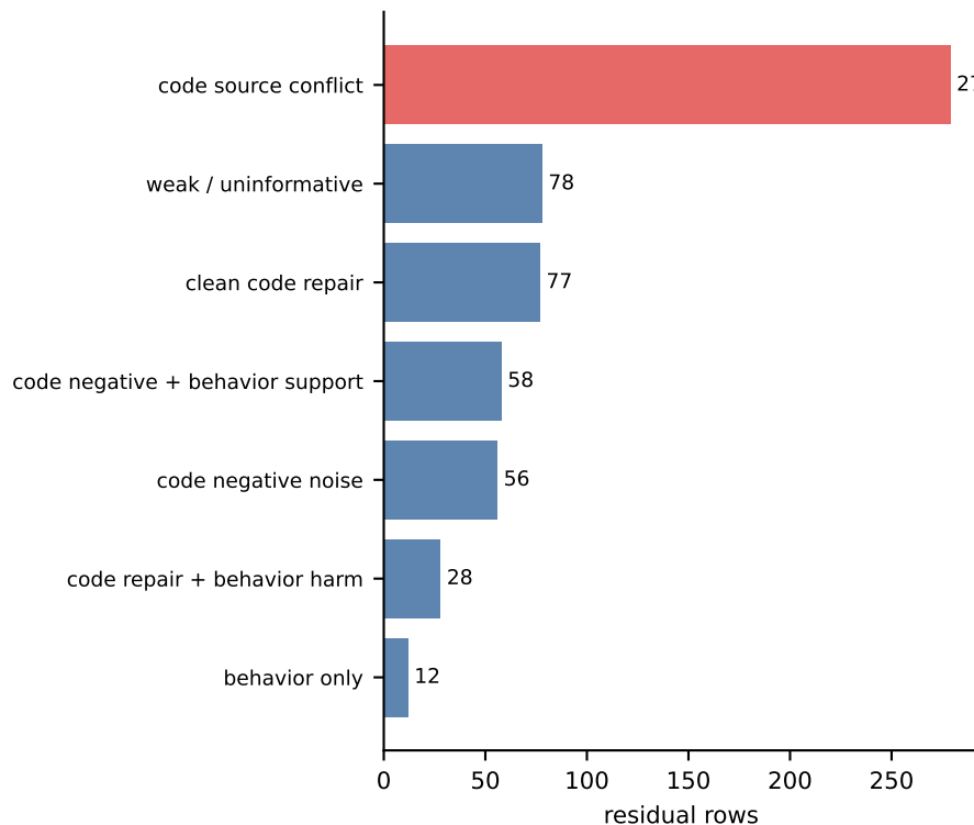
B. Most residual rows are conflict or weak evidence
