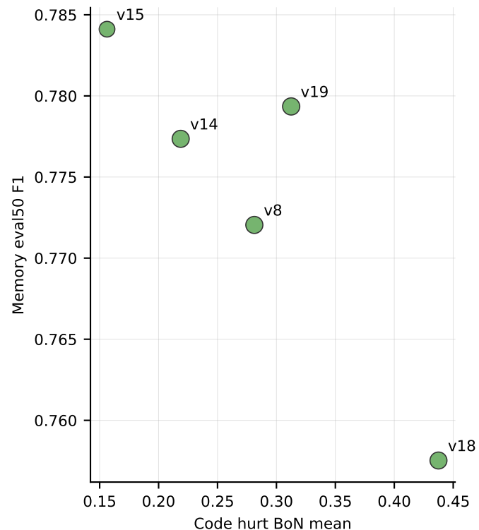
C. Rules expose a Memory-Code trade-off
