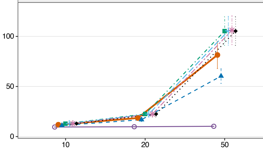
Random-slope model (RS)
