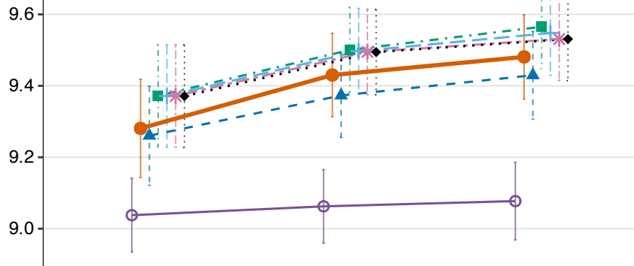
Random-slope model (RS)
