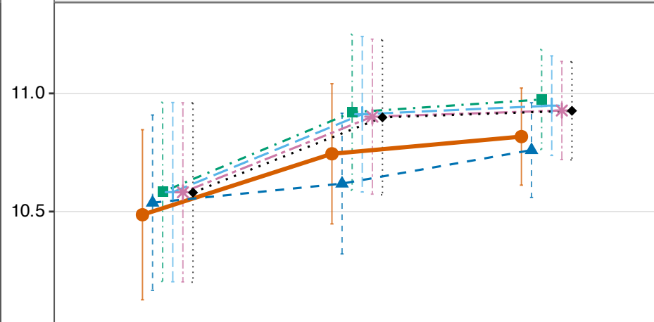
Random-slope model (RS)
