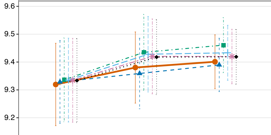
Random-slope model (RS)
