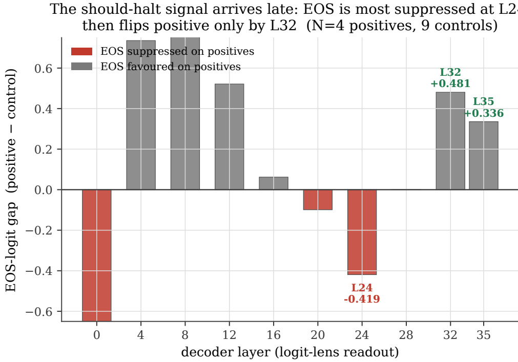
Figure 4: Logit-lens EOS-logit gap (positive minus control) by decoder layer. The gap is most negative at L24 ( -0.419 ), meaning EOS is most suppressed there, then flips positive to +0.481 at L32 and +0.336 at L35. The should-halt signal becomes legible at the unembedding only in the final layers, after the continuation state is committed upstream ( N = 4 positives, 9 controls).
