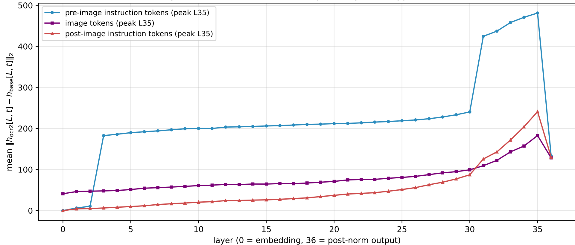
Figure 1d — Residual-diff decomposed by token type (N=26)
