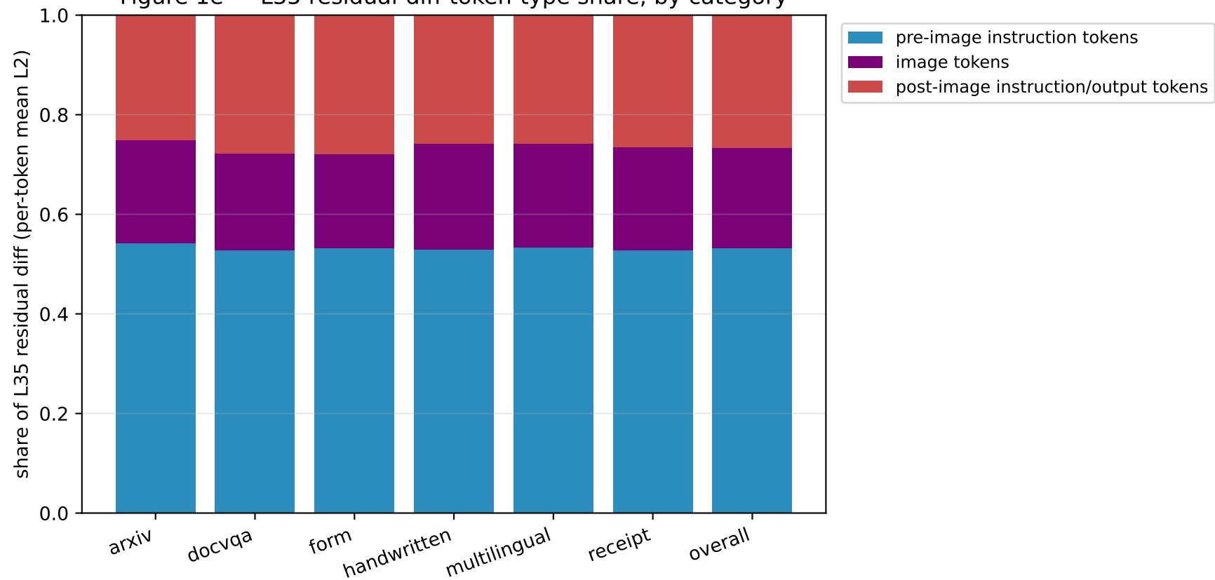
Figure 1e — L35 residual-diff token-type share, by category
