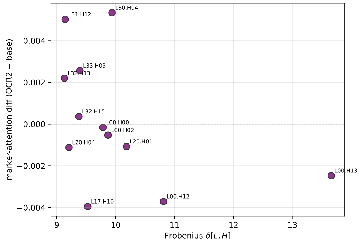
B. Top-12 Frobenius heads: are they also marker-attending?
