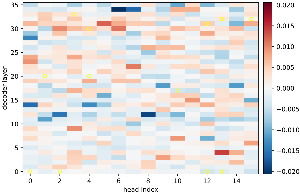
A. OCR2 – base attention to structured-marker tokens
