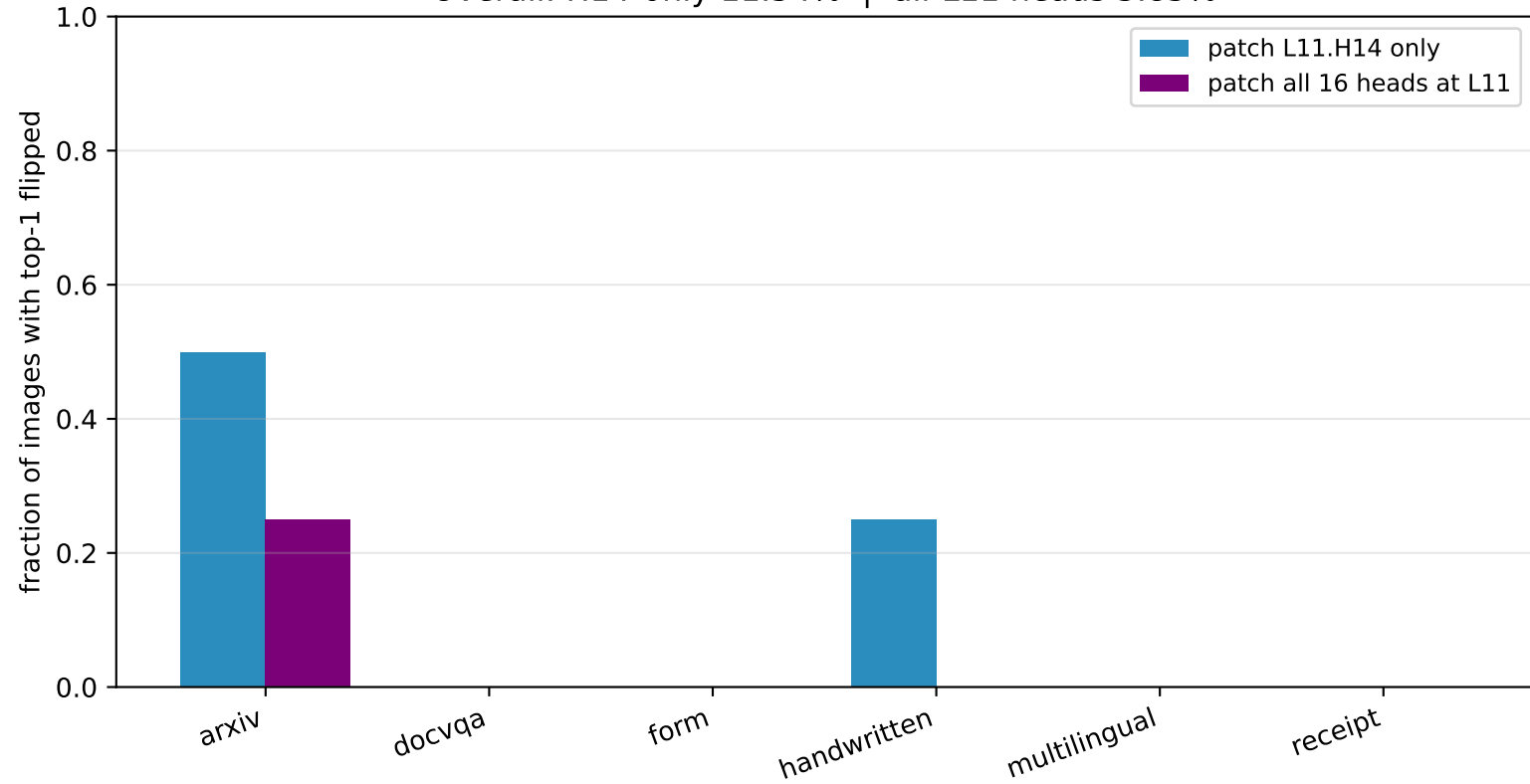
Figure 6 — L11 head-level patching: is L11.H14 (Hua router) load-bearing?
