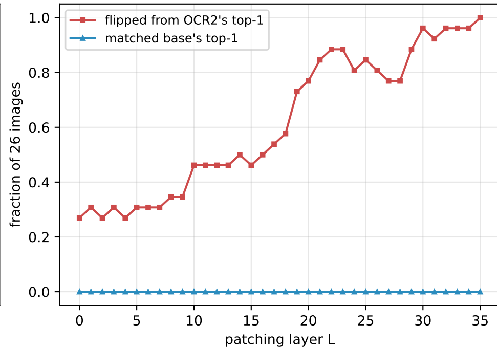
B. Reverse flip / base-match rate
