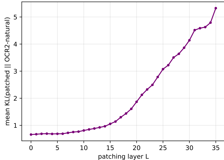
A. Mean KL at last position base residual injected at L, OCR2 continues
