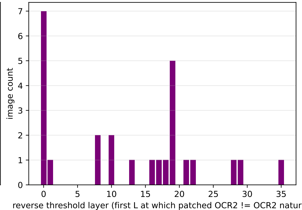
C. Per-image reverse threshold distribution median L=14, mode L=0
