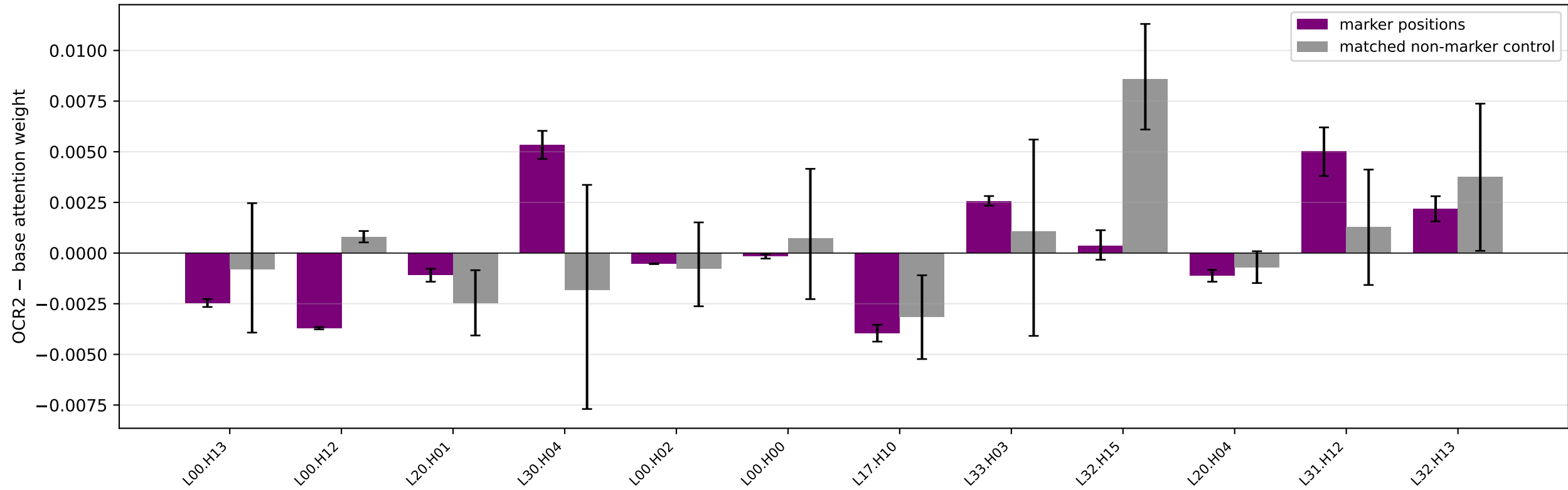
Top-12 Frobenius heads — marker attention vs non-marker control Bootstrap 95% CI over N=26 images, 1000 resamples
