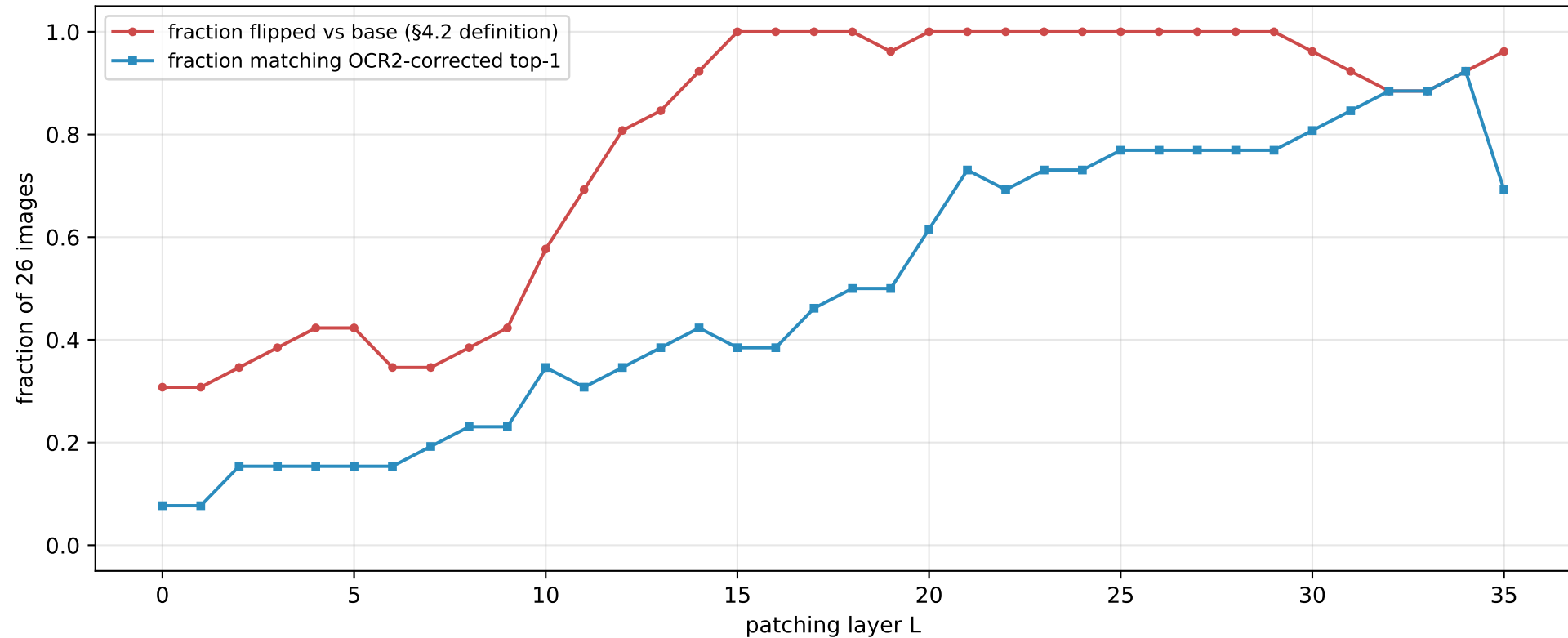
Forward patching: flip-vs-base (§4.2) vs match-OCR2-corrected Peak match rate 92.3%, L35 match rate 69.2%
