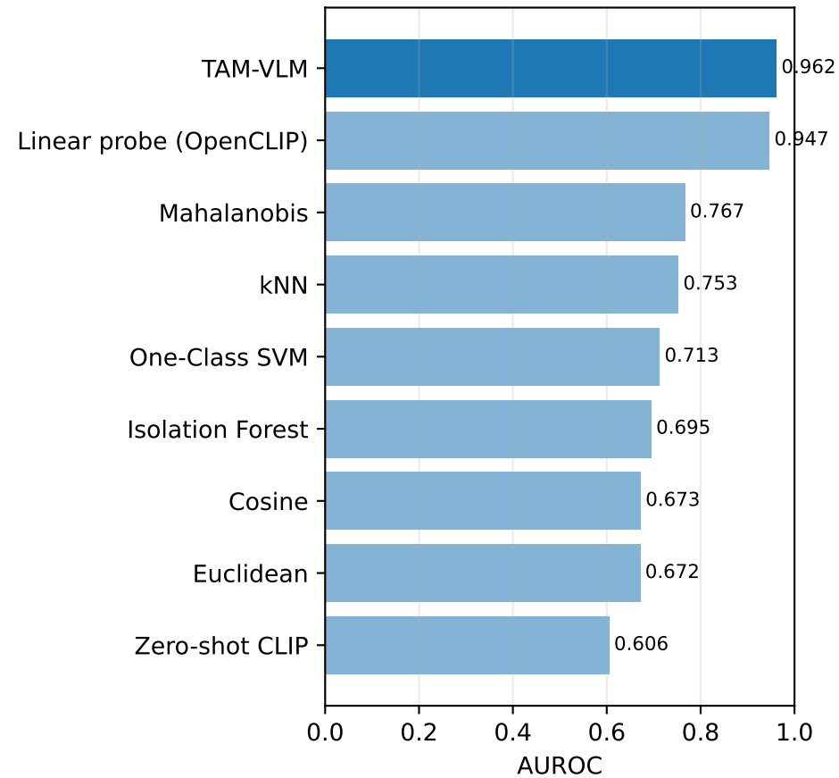
OpenCLIP ViT-B/16
