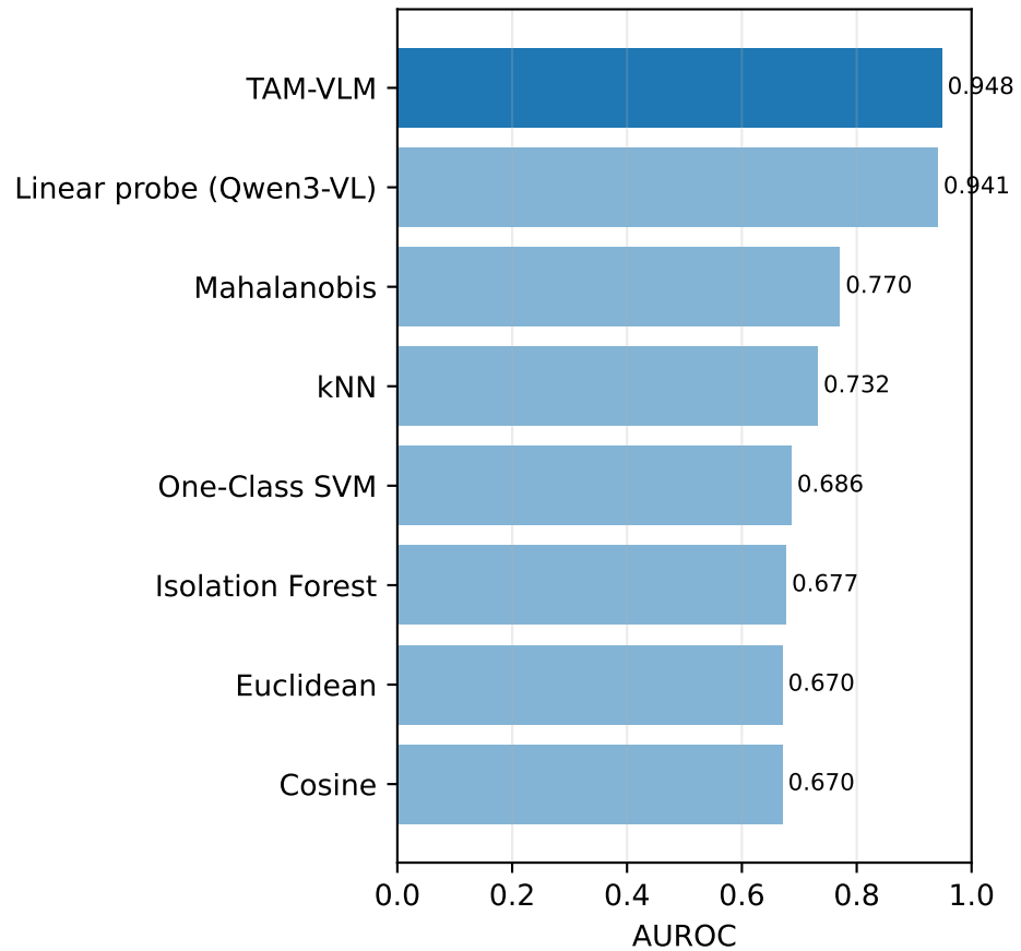
Qwen3-VL-Embedding-2B
