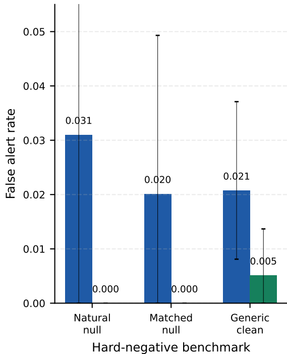
(b) Hard-negative false alert rate
