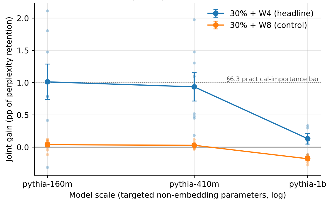
Joint gain against model scale
