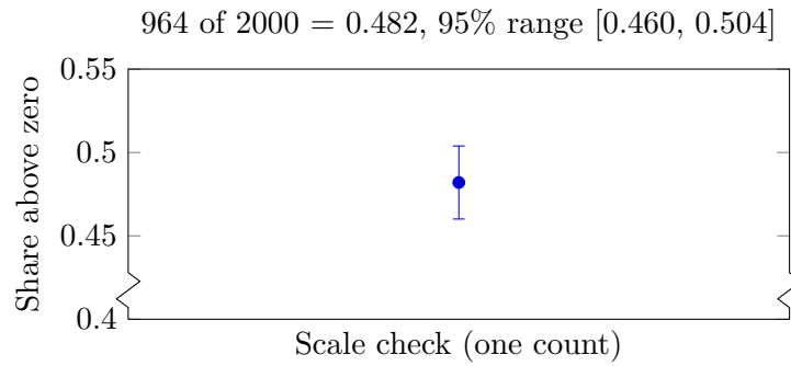
Figure 2: Scale check (axis break: point starts at 0.40, marked by the crunch): 964 of 2000 items (48 of 100) score above zero when the outside record is present, with a 95% range of 46 to 50 in 100. Seven of seven present-above-mixed confirmations (range about 65 to 100 in 100). Share above zero means items scoring above zero divided by all items.
