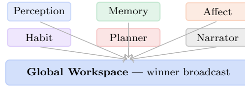
Figure 7: The parliament at mind scale: 6 parties bid via salience × utility; winner broadcast globally, experienced as “my thought” 200 ms after competition. No captain, configuration votes. This is Layer 4, the global workspace where coalition competition becomes conscious access.
