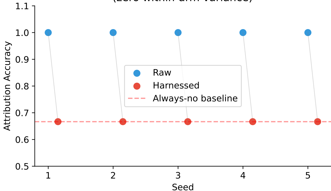
Per-Seed Attribution: Raw vs Harnessed (zero within-arm variance)
