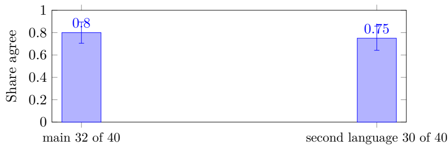
Figure 4: Failure-mode agreement plotted (not only captioned): main 32 of 40 checks agree (80 of 100, range 65 to 90) and second language 30 of 40 (75 of 100, range 60 to 86). Agreement means checks where all wirings give the same confident-wrong answer.
