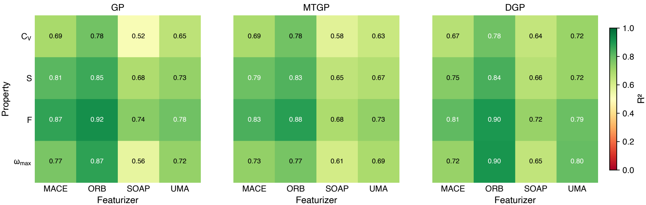
Phonon (Pheasy) — R^2 heatmap ( n_{\text{train}} = 500 , best PCA per surrogate)
