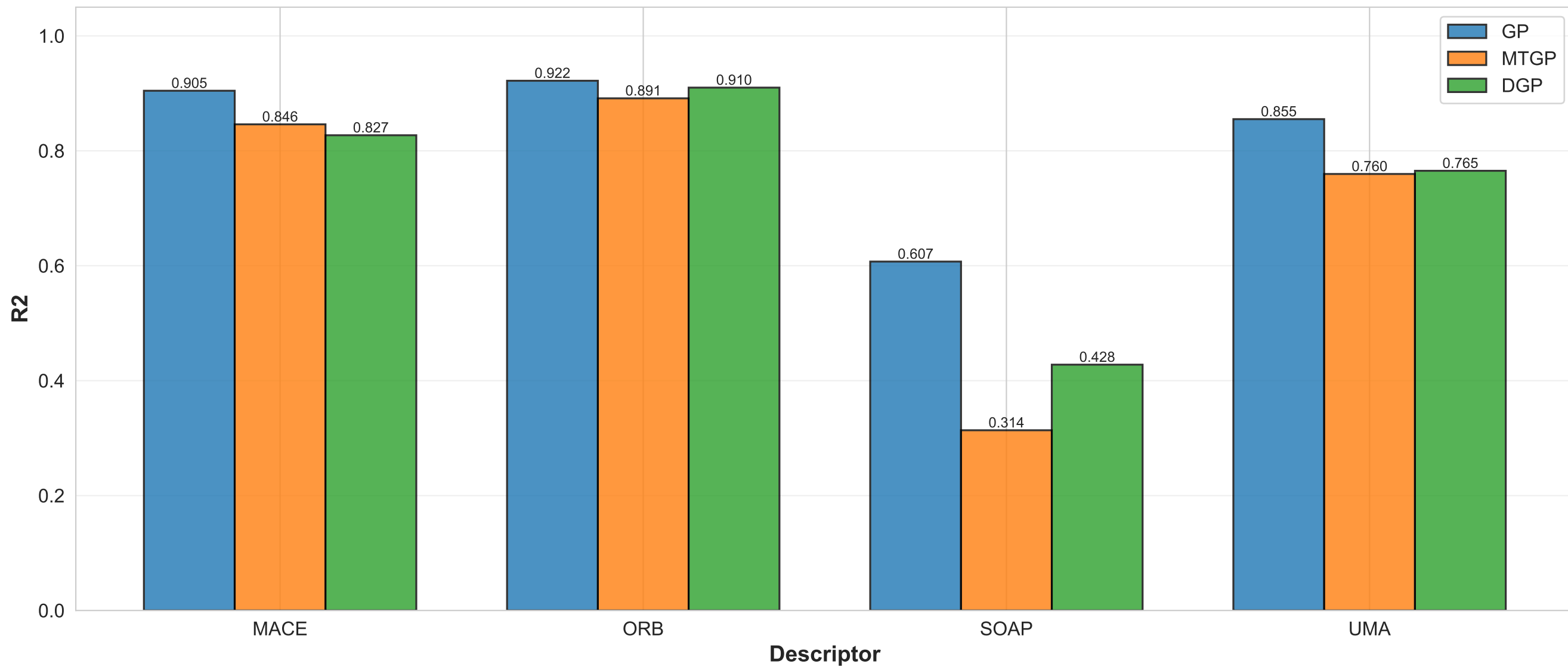
K_VRH: R2 (n=500, Best PCA per Surrogate for This Property)
