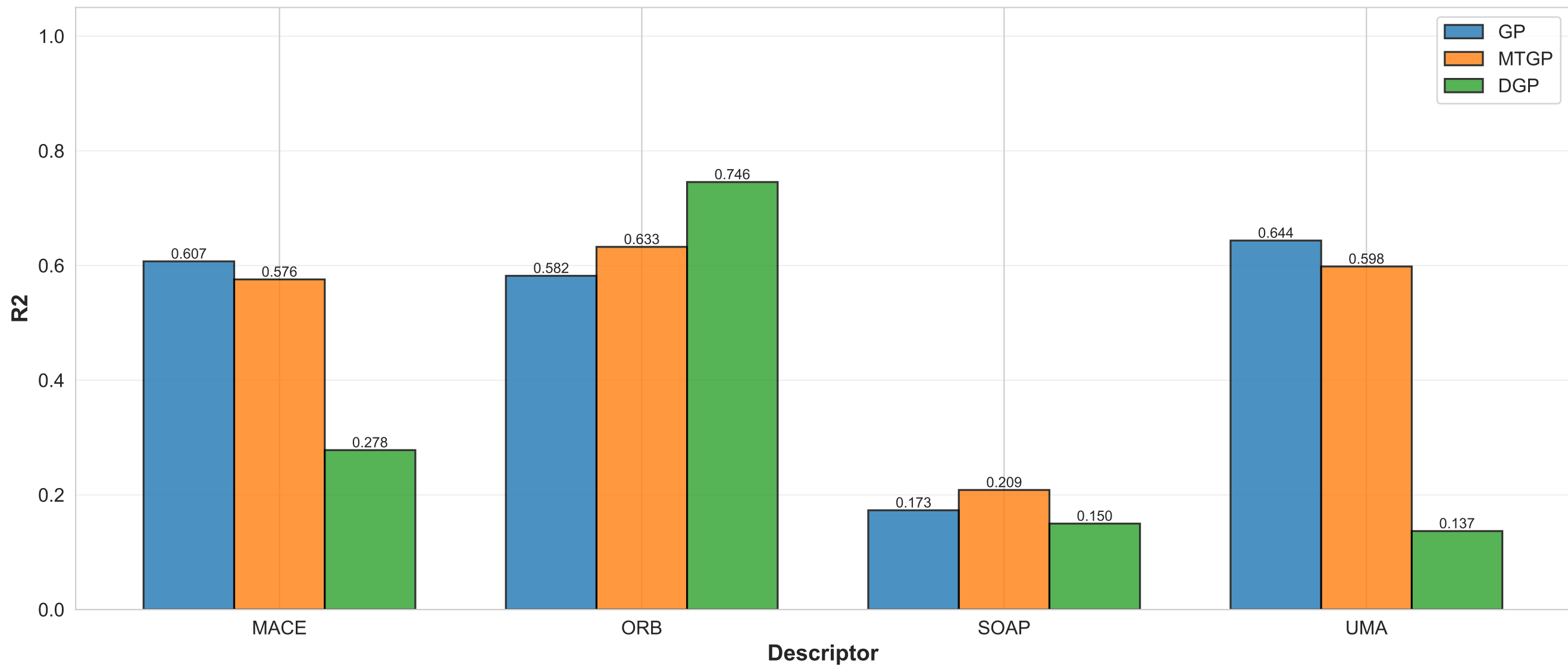
elastic_anisotropy: R2 (n=500, Best PCA per Surrogate for This Property)
