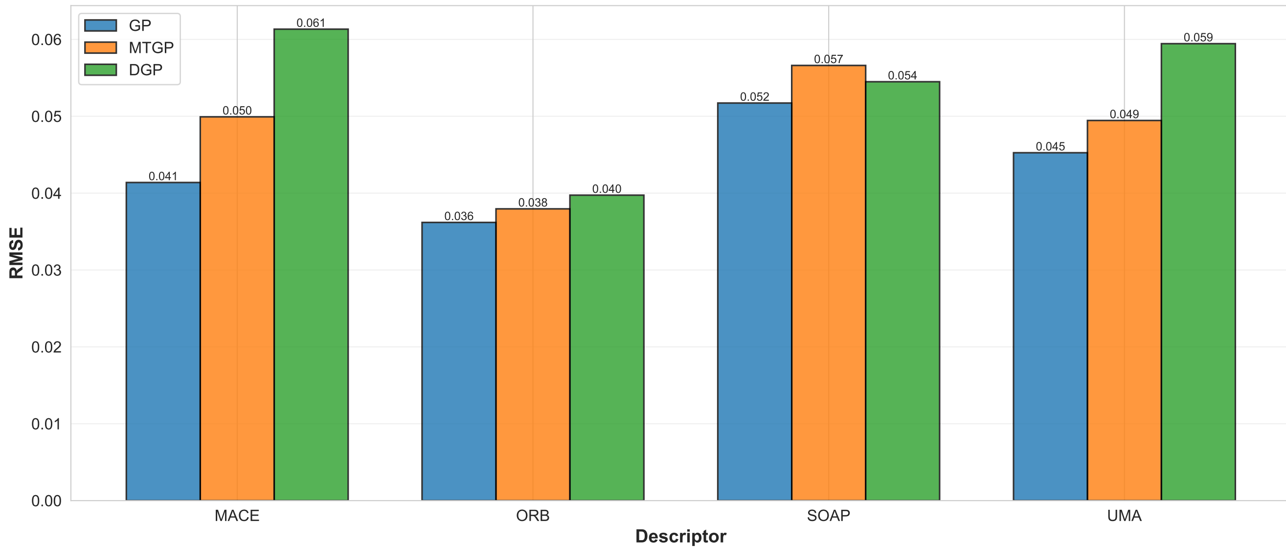
poisson_ratio: RMSE (n=500, Best PCA per Surrogate for This Property)
