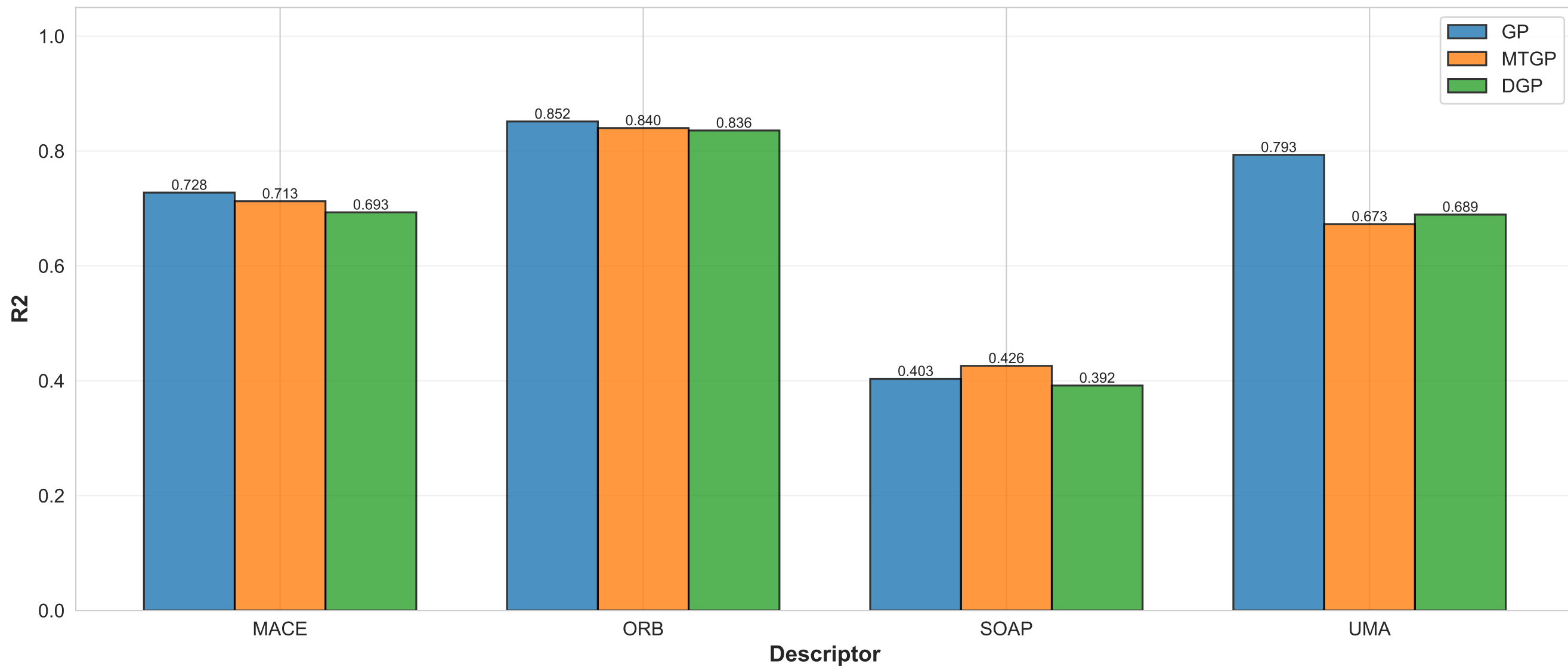
band_gap: R2 (n=500, Best PCA per Surrogate for This Property)
