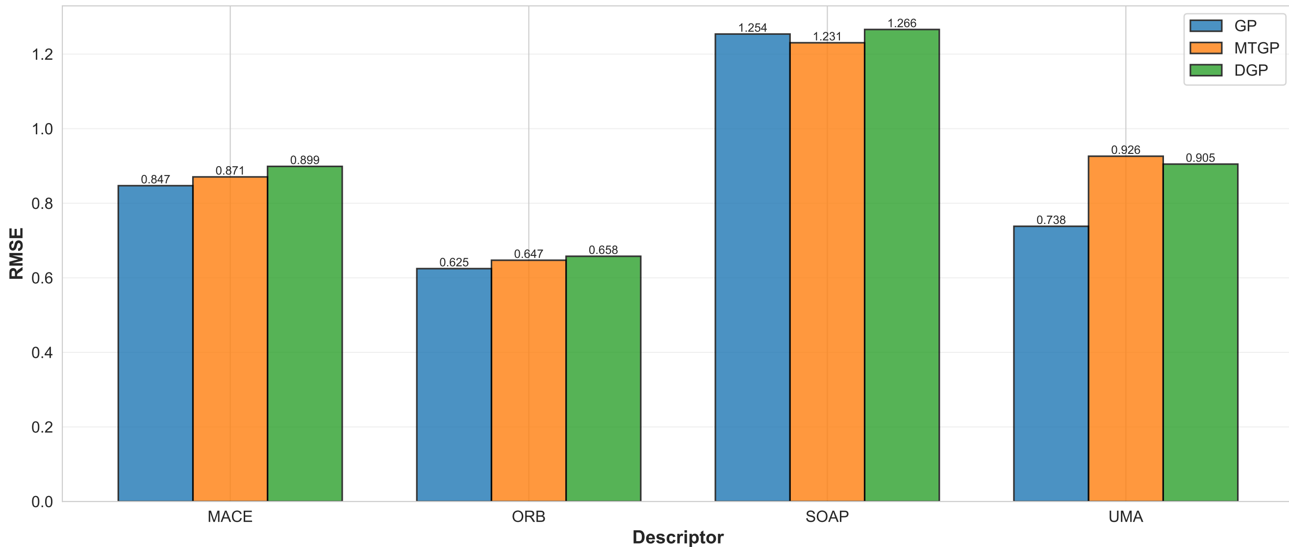
band_gap: RMSE (n=500, Best PCA per Surrogate for This Property)
