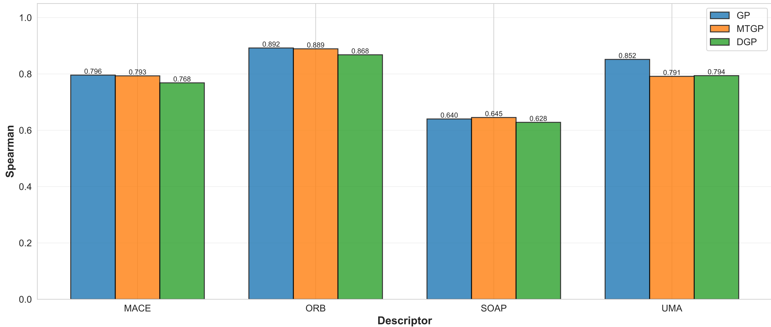
band_gap: Spearman (n=500, Best PCA per Surrogate for This Property)
