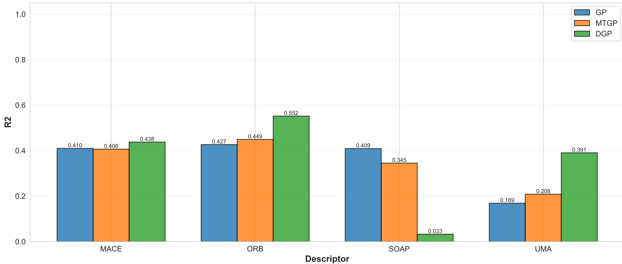
n: R2 (n=500, Best PCA per Surrogate for This Property)
