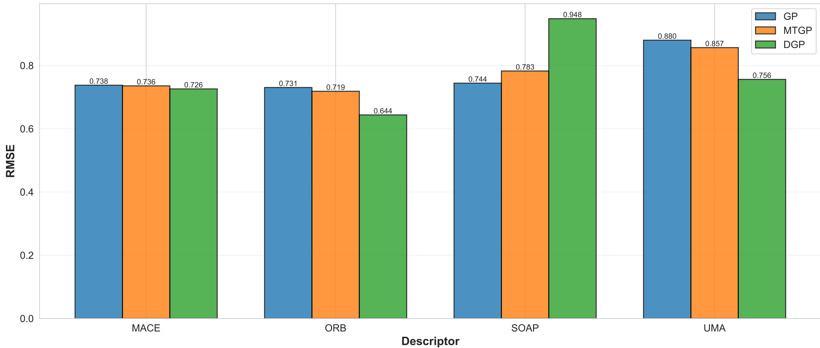
n: RMSE (n=500, Best PCA per Surrogate for This Property)
