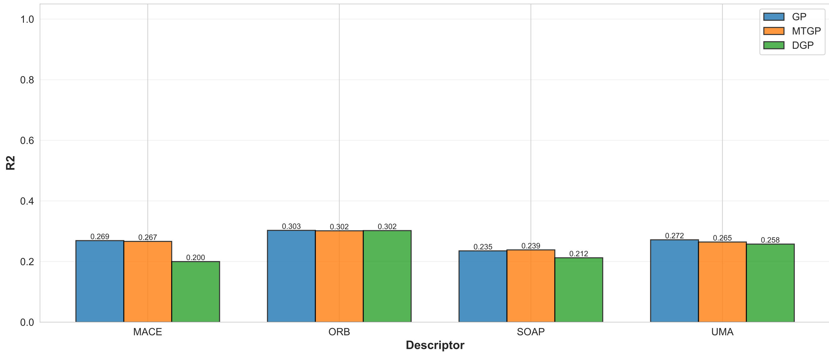
Averaged R2 Across Properties (n=500, Best PCA per Surrogate)
