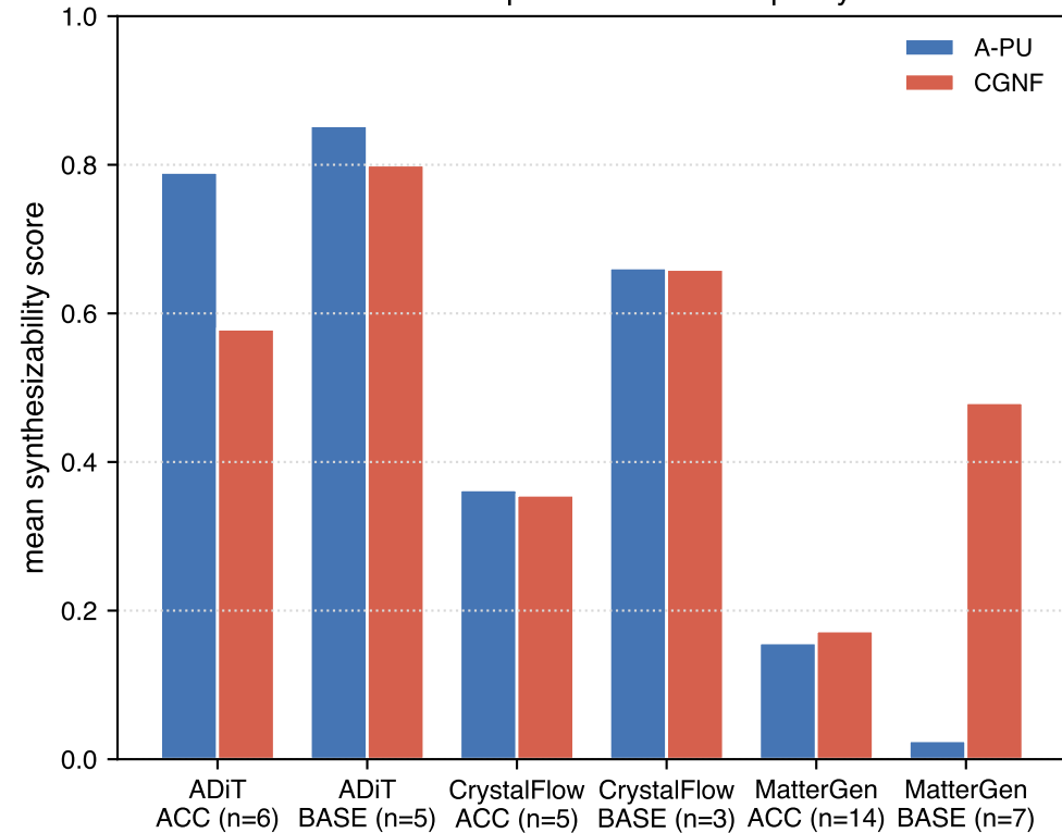
Mean score per backbone and policy
