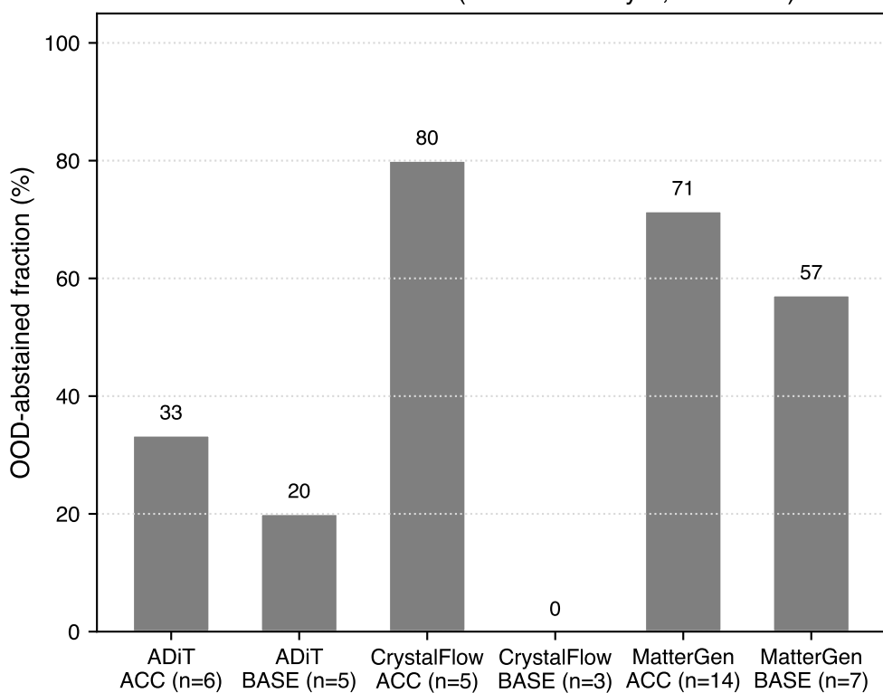
Out-of-distribution rate (A-PU OOD layer, corrected)
