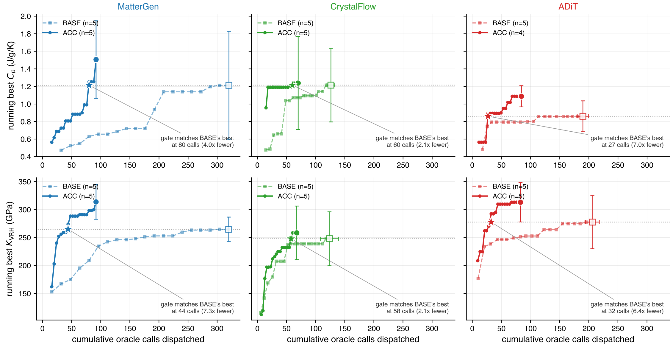
Discovery vs oracle cost per backbone (5-seed mean; endpoint \pm std; * = gate reaches ungated policy's final best)
