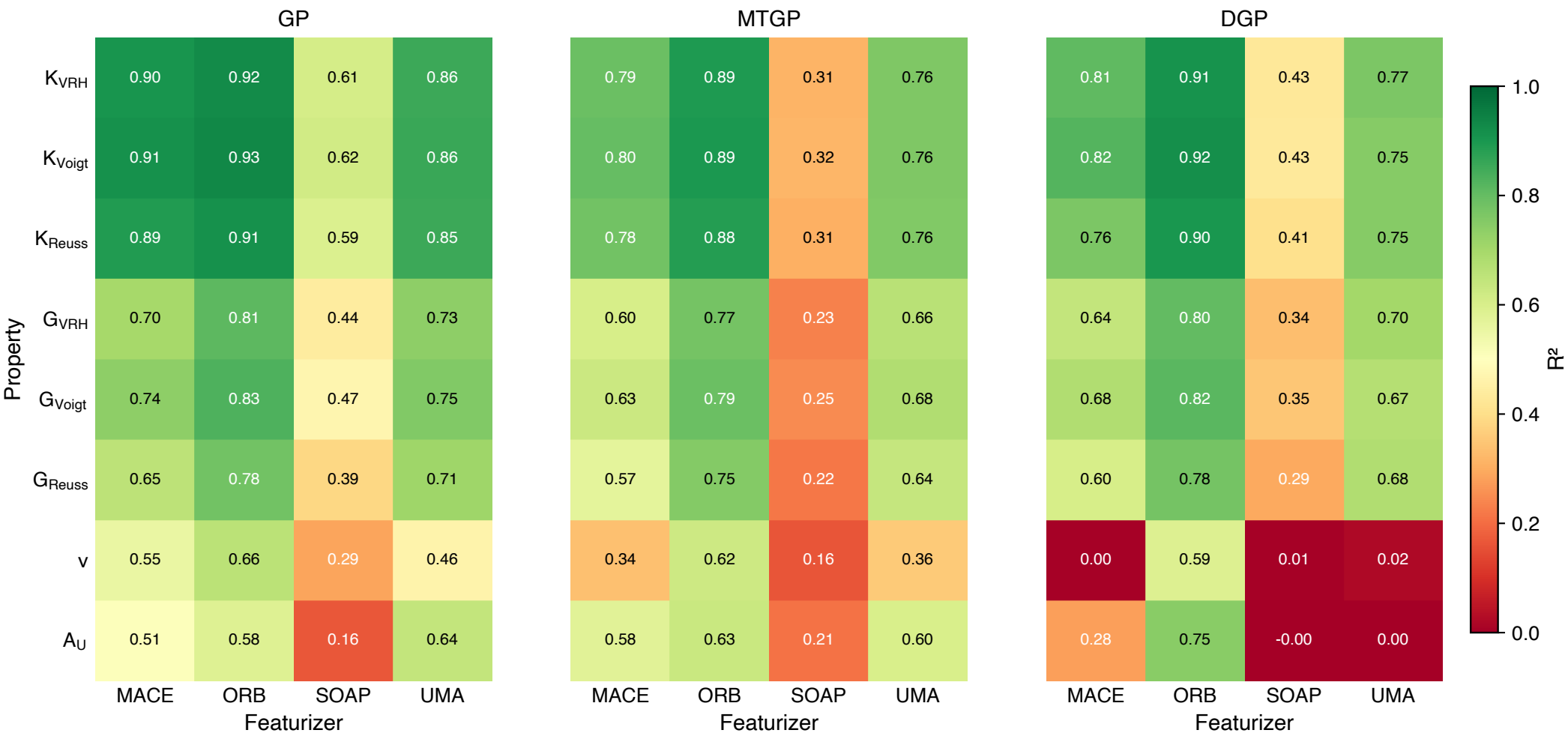
Elastic — R^2 heatmap ( n_{\text{train}} = 500 , best PCA per surrogate)
