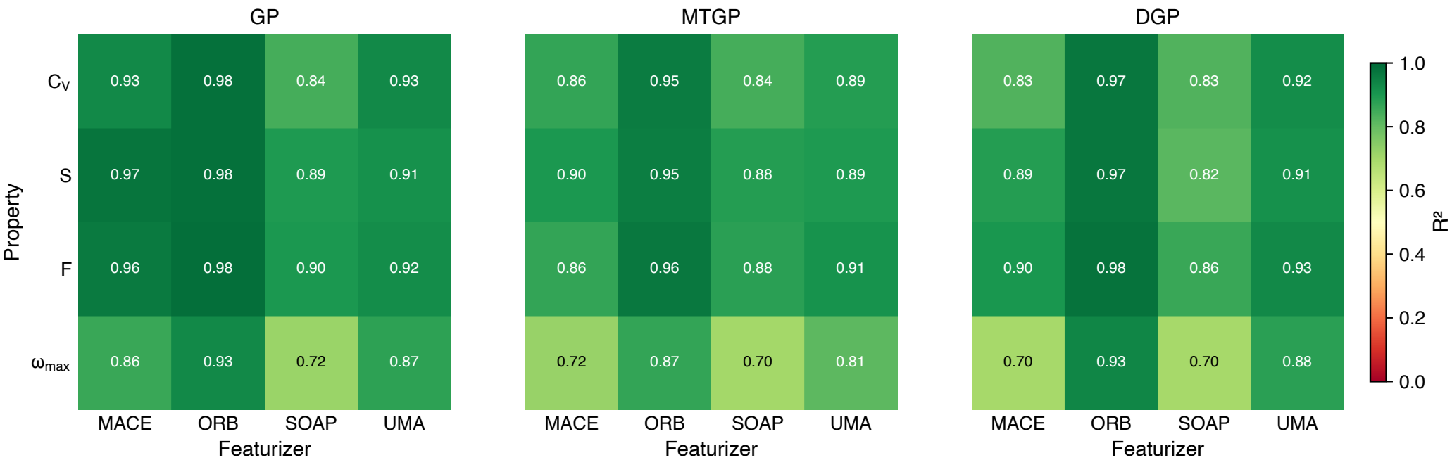
Phonon — R^2 heatmap ( n_{\text{train}} = 500 , best PCA per surrogate)
