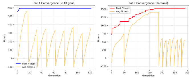
Fig. 1. Fitness convergence over generations. Left: Rapid convergence on Pot A. Right: Prolonged plateauing on Pot E, with periodic crashes in average fitness due to mass extinction events.
