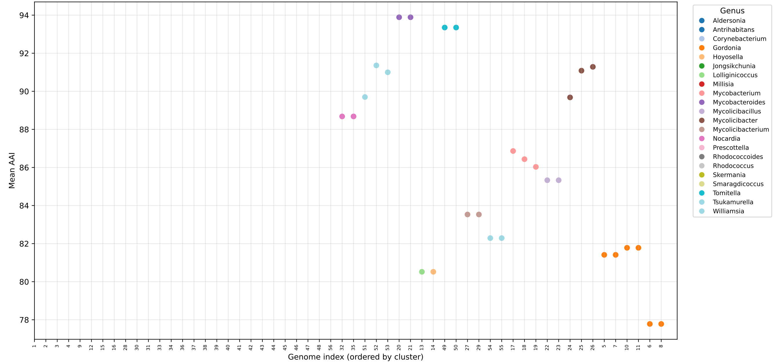
Per-genome mean AAI within cluster
