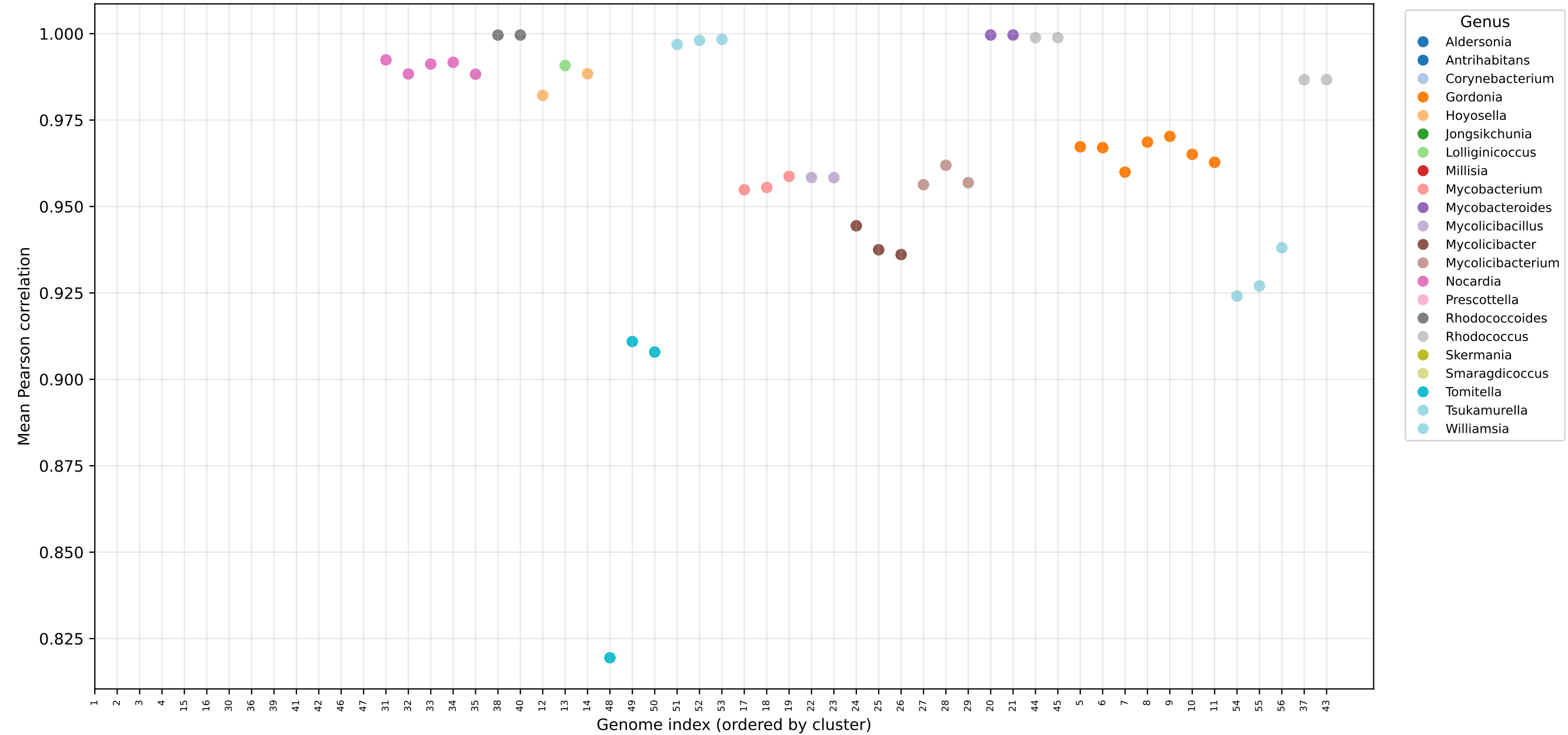
Per-genome mean Pearson correlation within cluster
