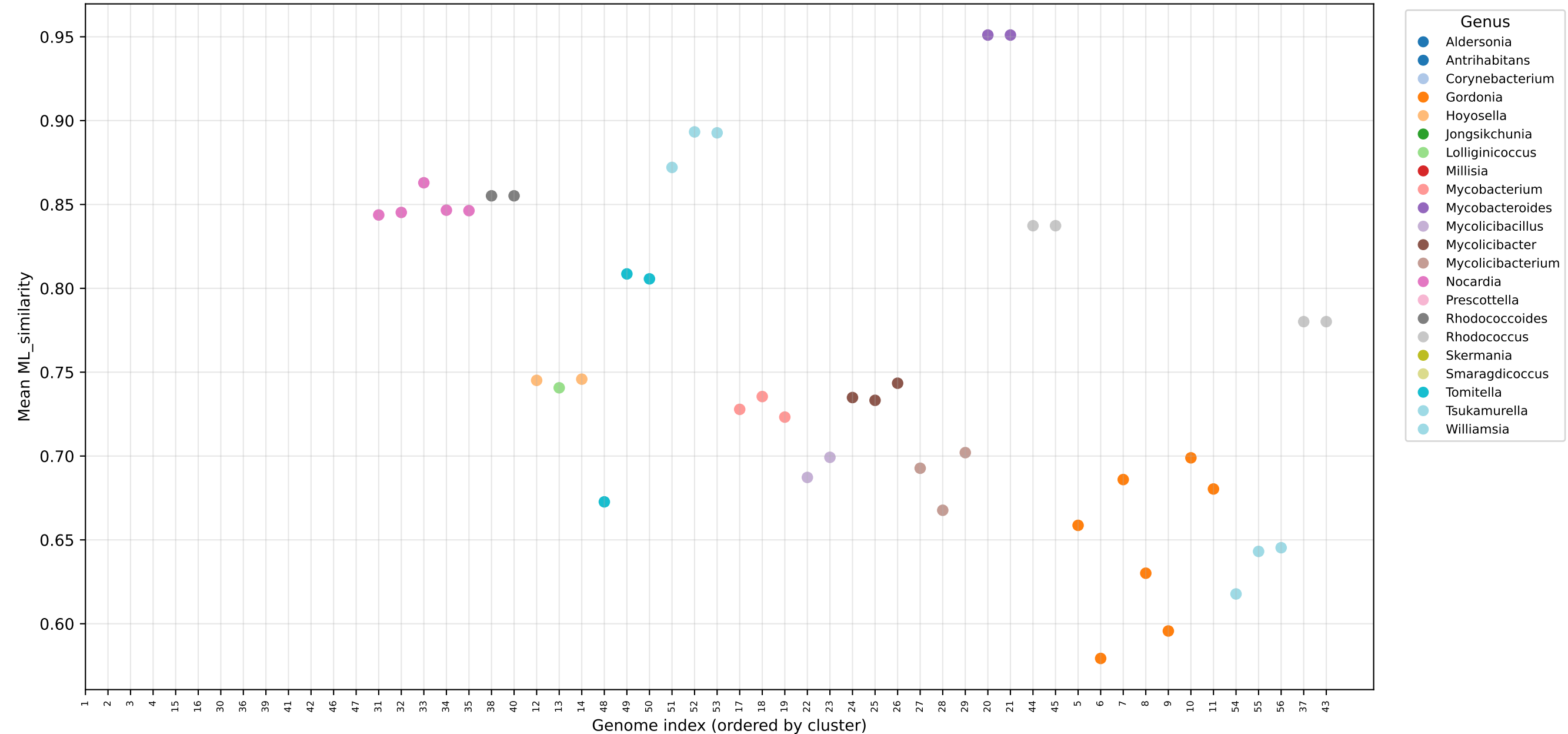
Per-genome mean ML_similarity within cluster
