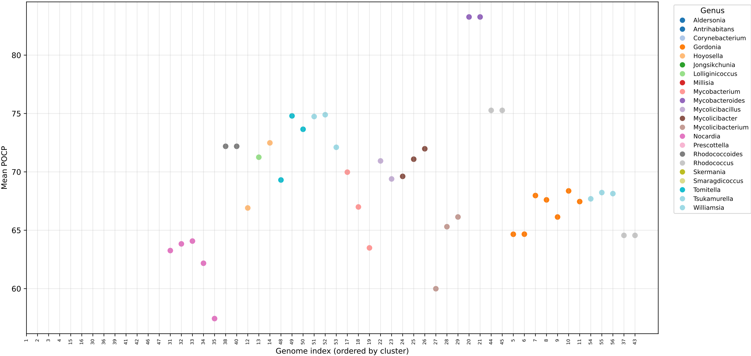
Per-genome mean POCP within cluster
