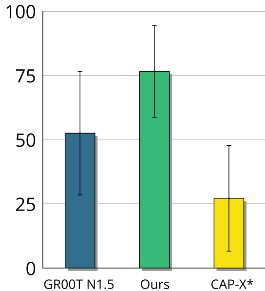
OpenStandMixerHead
