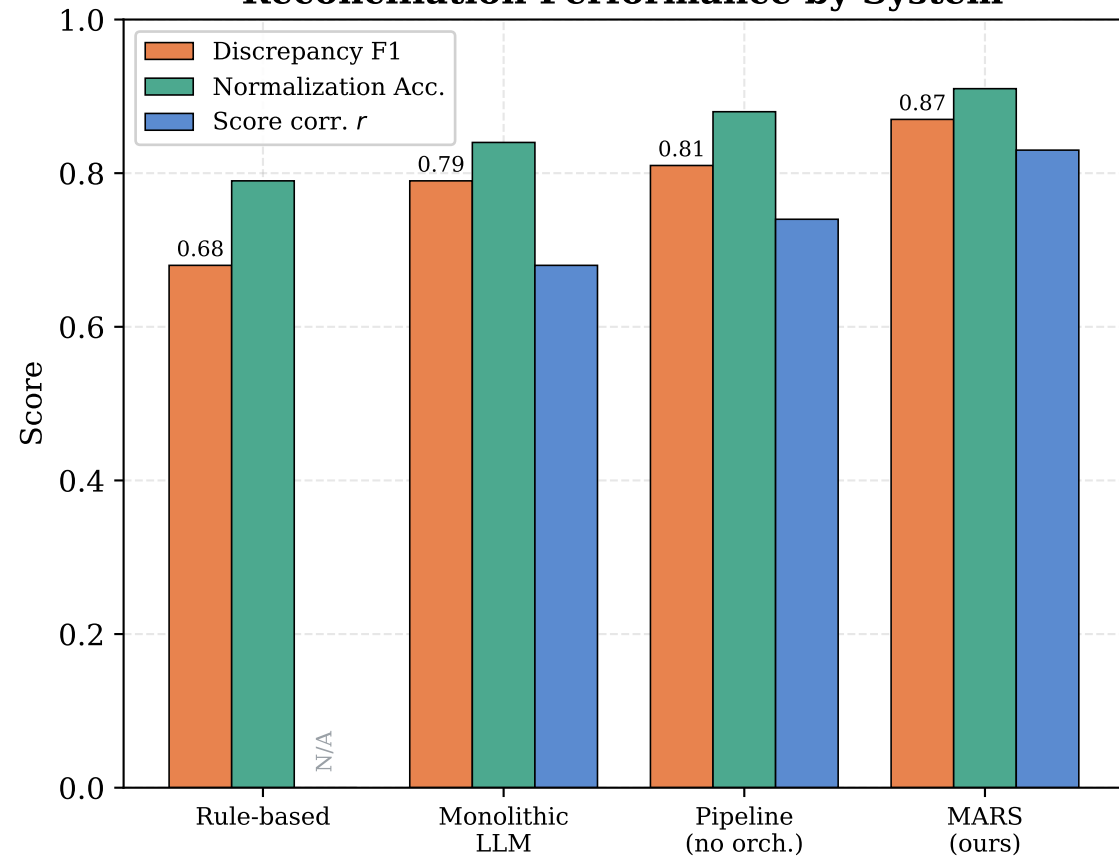
Reconciliation Performance by System
