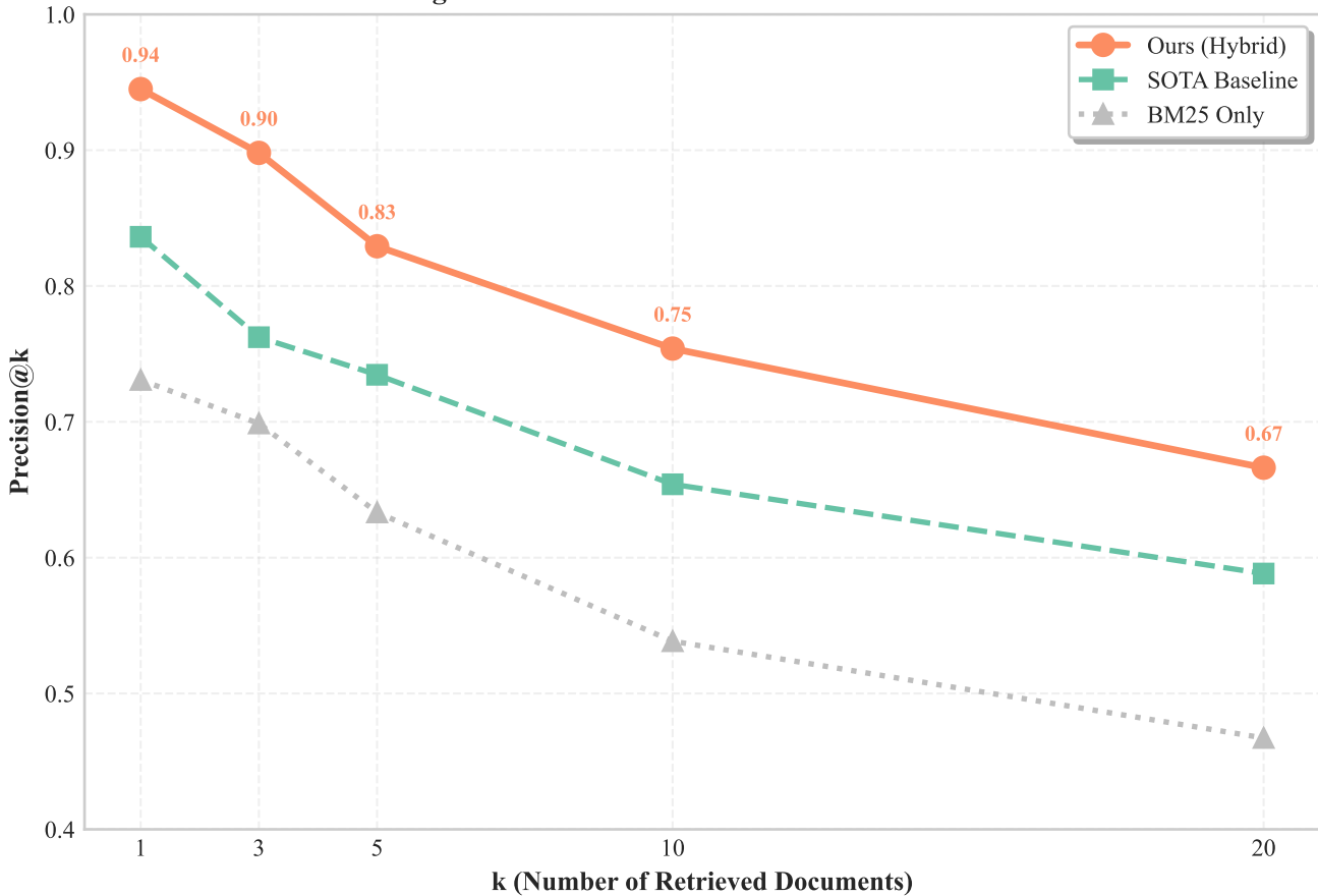
Fig 6: Retrieval Precision at Different k Values
