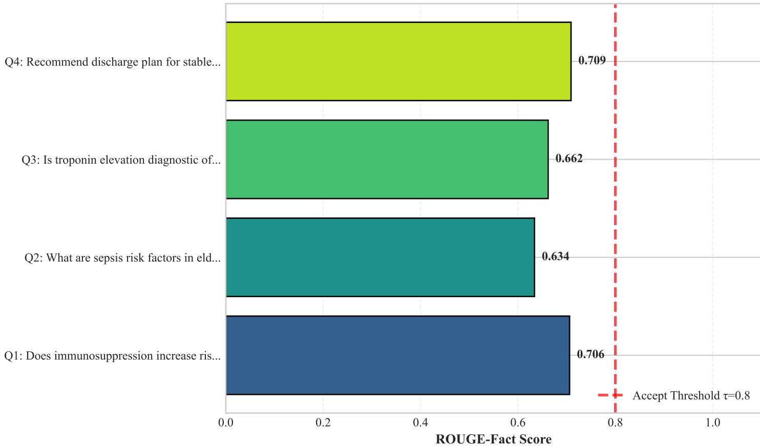
Fig 3: Factual Consistency per Query
