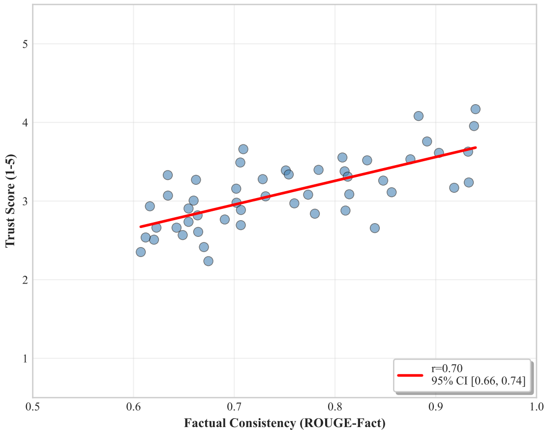
Trust vs. Factual Consistency Correlation
