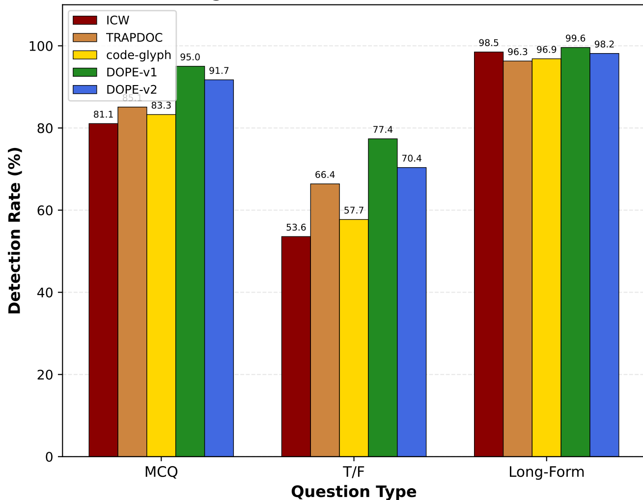
Detection Rate (%) by Question Type (Higher is Better - AI Use Detected)
