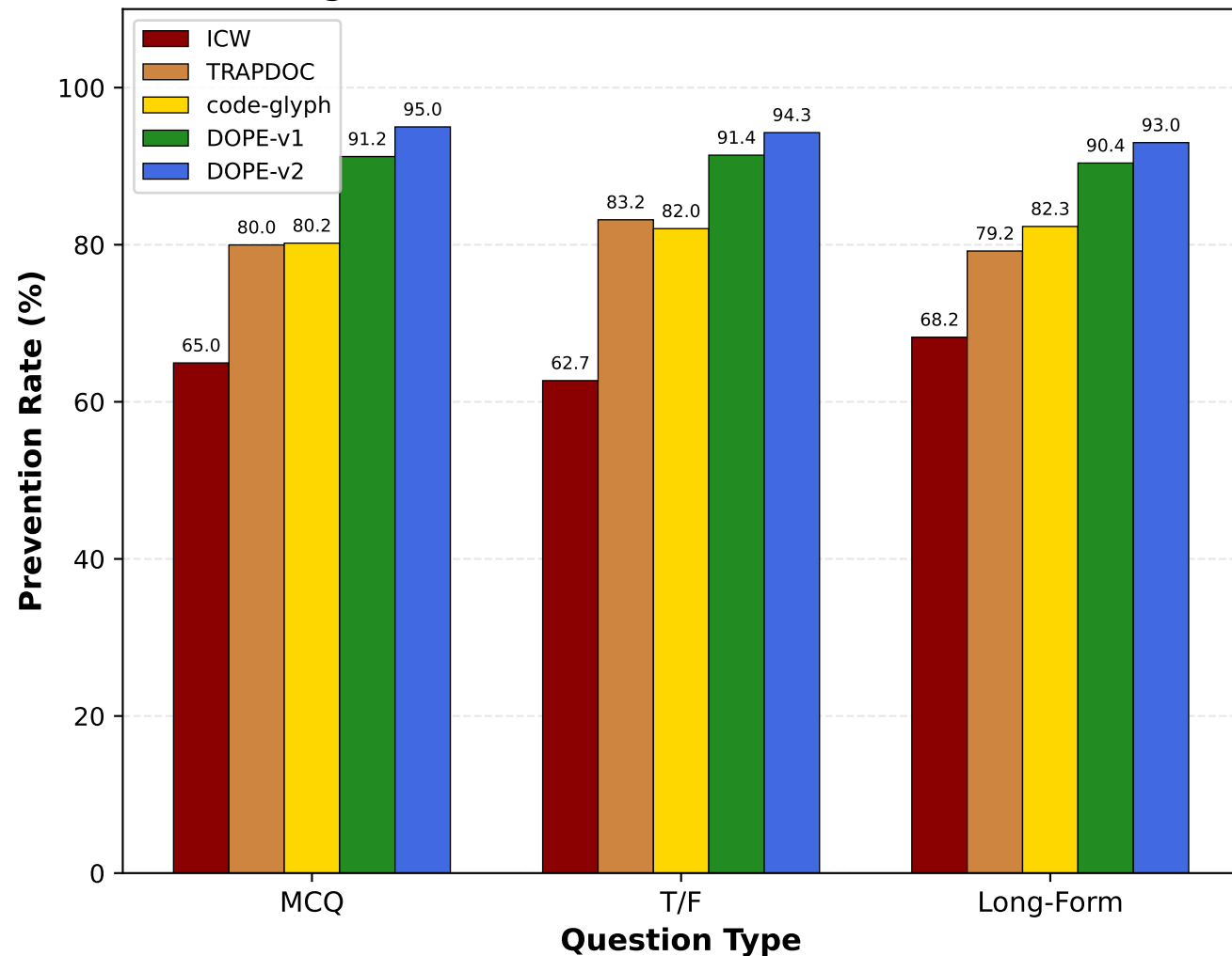
Prevention Rate (%) by Question Type (Higher is Better - Model Refuses to Answer)
