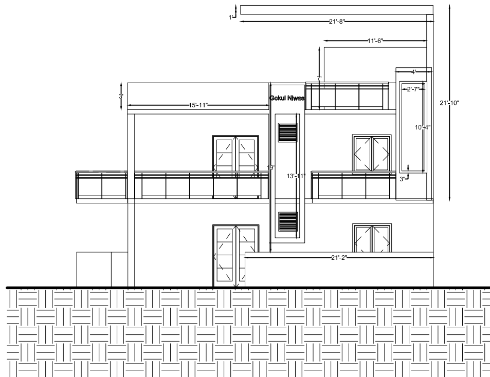
ELEVATION VIEW
