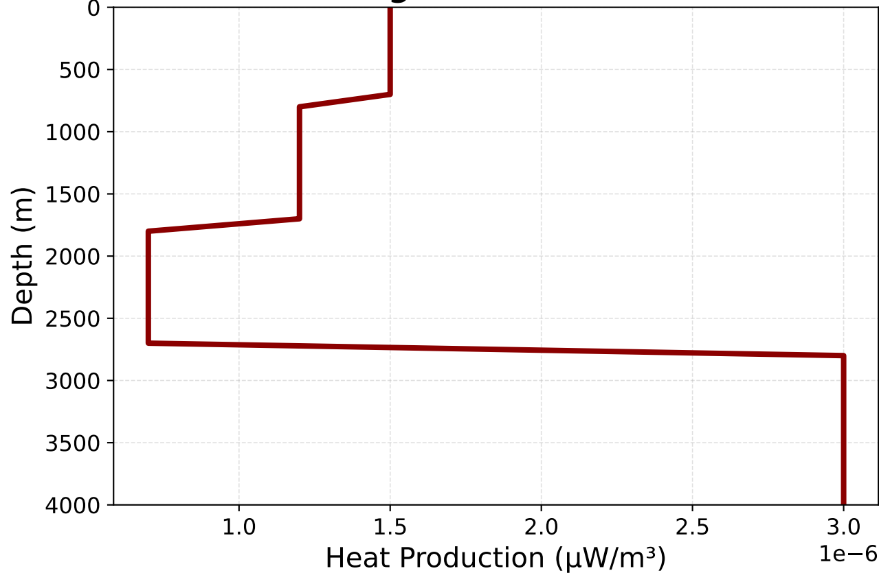
Radiogenic Heat Profile
