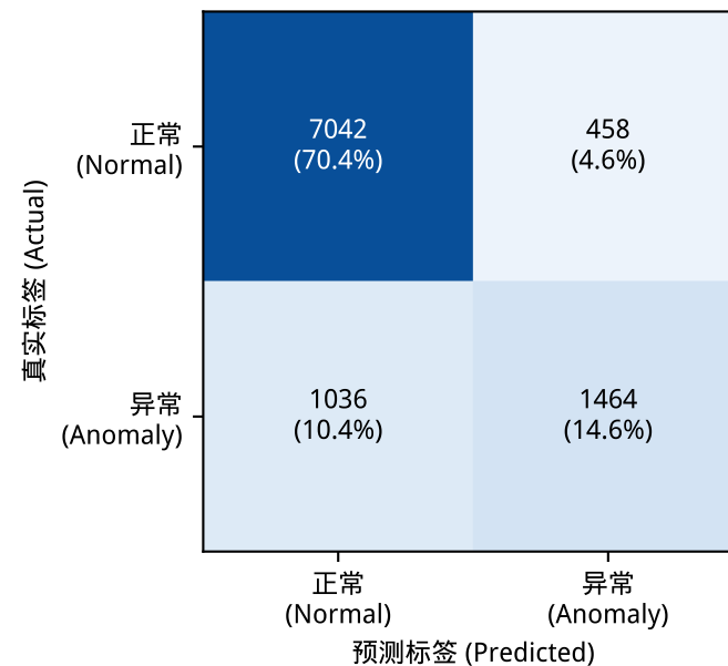
(c) V-TimesNet_v2
