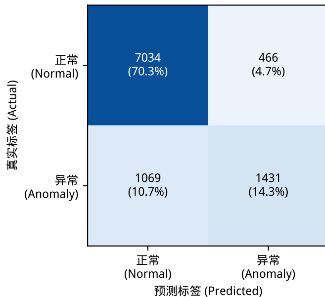
(b) V-TimesNet
