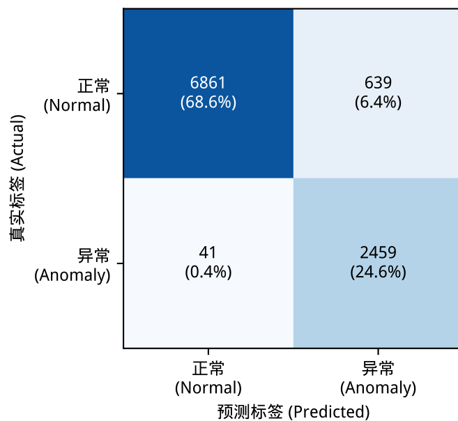
(e) DLinear
