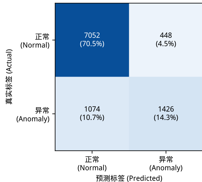
(a) TimesNet
