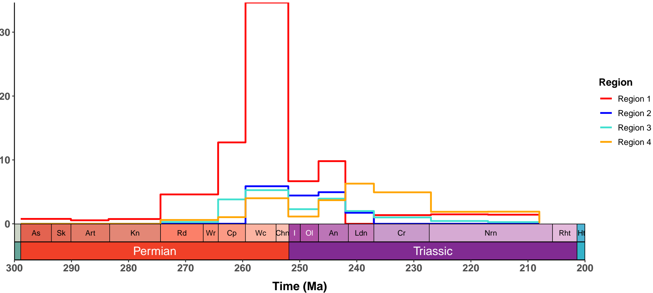
Diversity Through Time (# Genera) by Region
